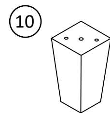
x4 T5042196100UD FOOT
